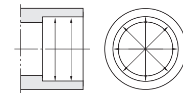
Fig. 15-2 Measuring points on housing bore diameter
