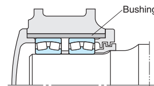
Fig. 14-1 Example of light alloy housing
