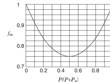
Fig. 5-12 Coefficient f_m
